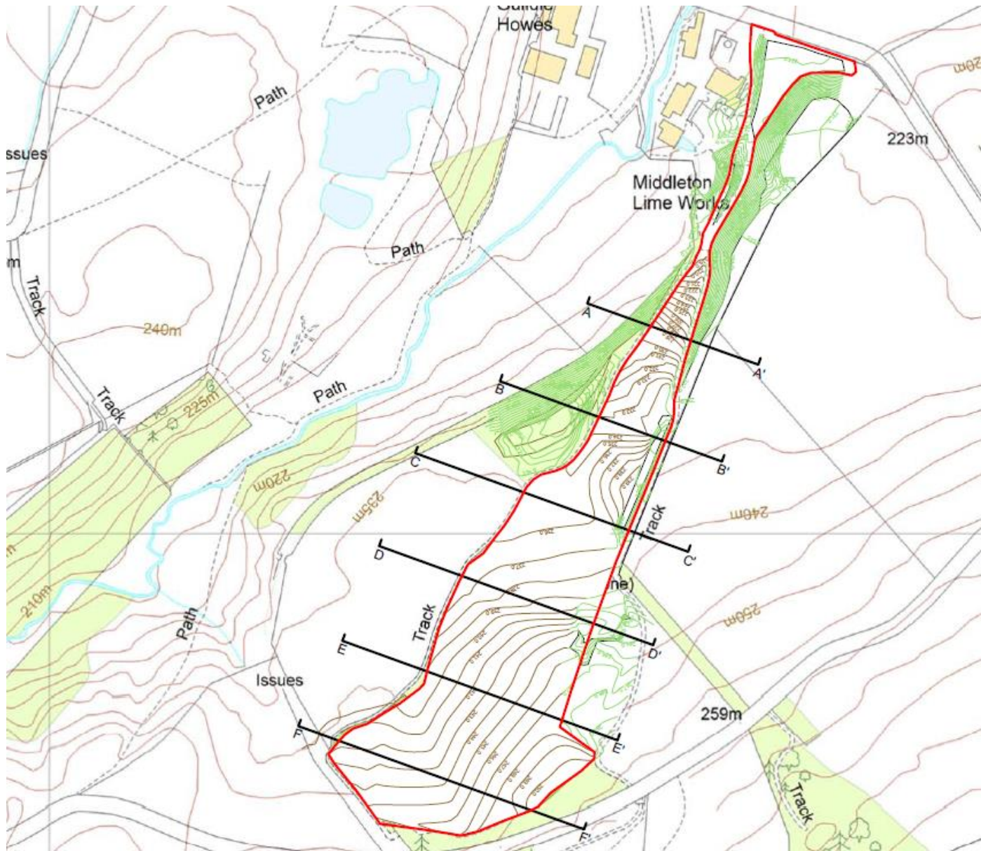
Restoration Contours
